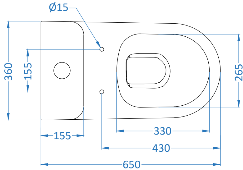
TOP VIEW
