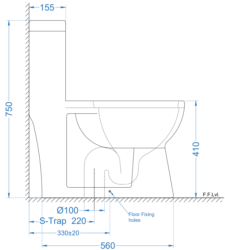
SIDE VIEW
