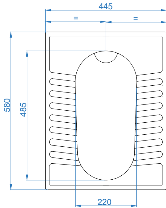
TOP VIEW
