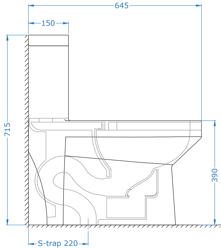
SIDE VIEW
